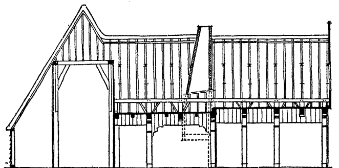
LANGSDOORSNED E-B.
